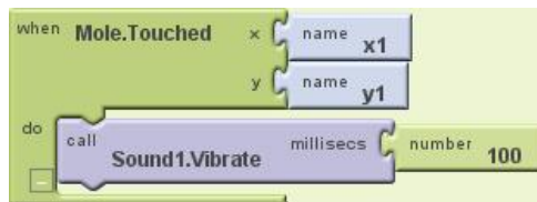
Figure 3-10. Making the phone vibrate briefly (for 100 milliseconds) when the mole is touched
